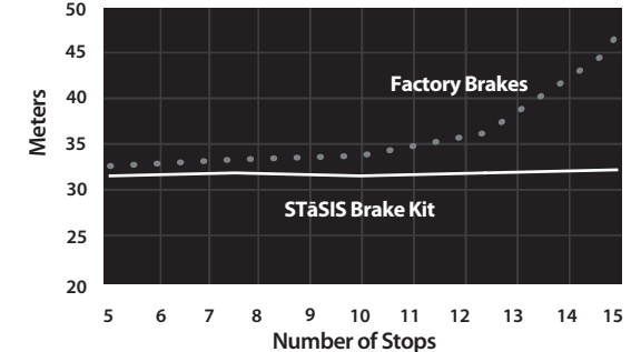
STOPPING DISTANCE OVER CONSECUTIVE STOPS FROM 100 KPH (62 MPH)
