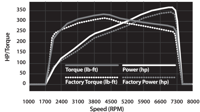
HORSEPOWER/TORQUE GAINS
