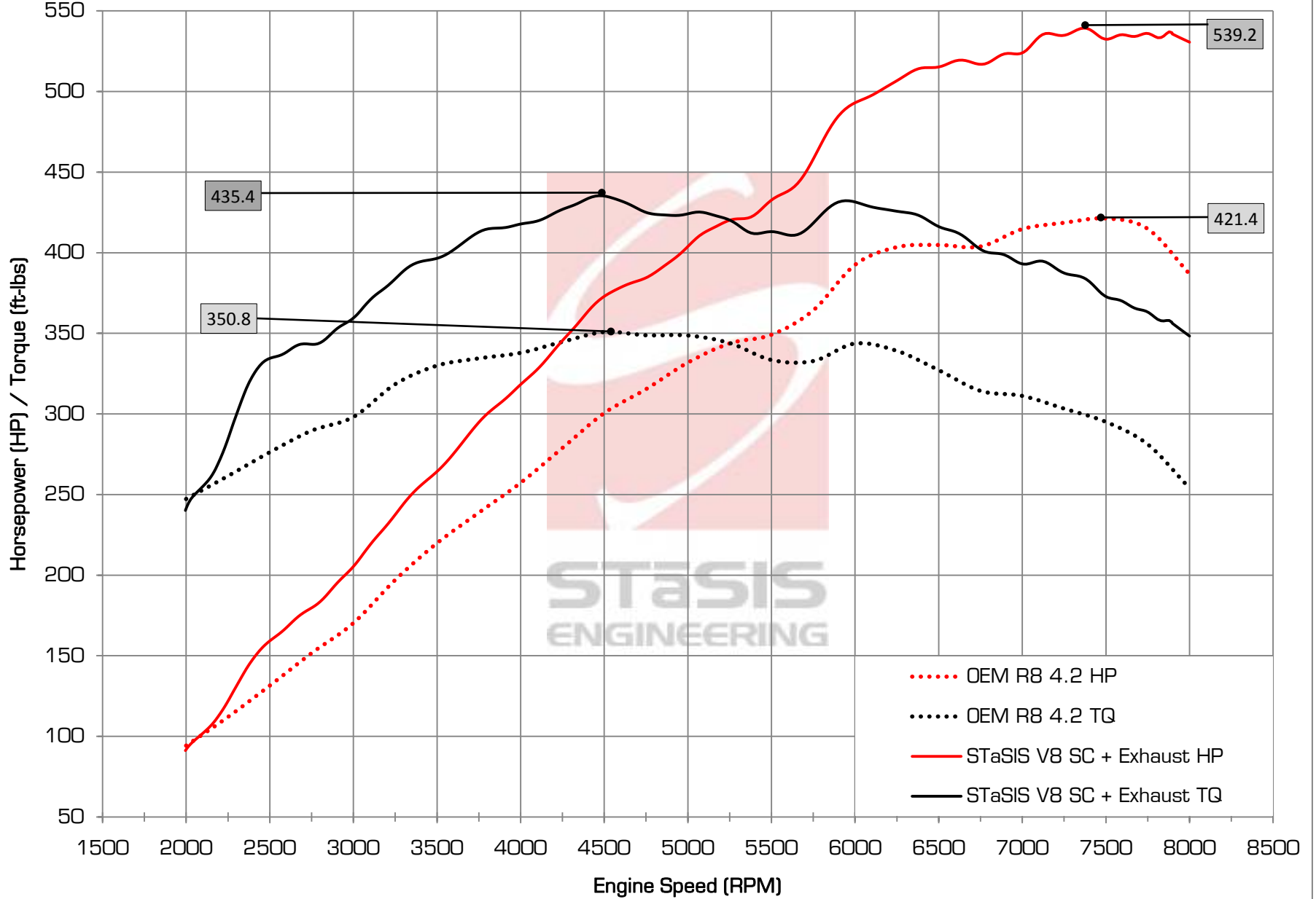
R8 4.2 STaSIS Supercharger Comparison - Crankshaft Power
