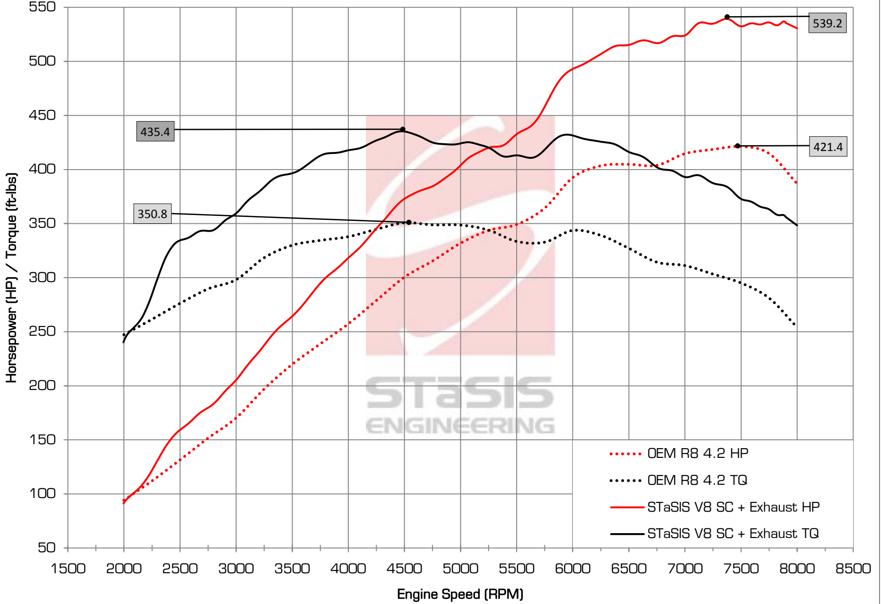
R8 4.2 STaSIS Supercharger Comparison - Crankshaft Power
