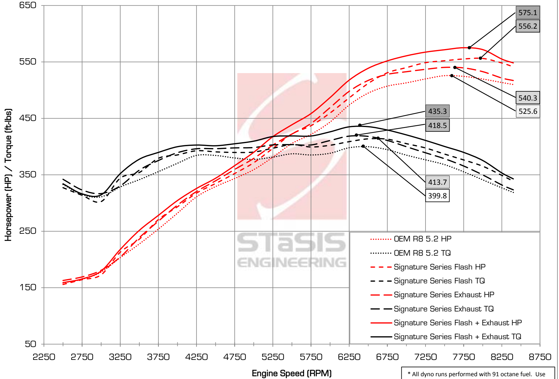
STaSiS Engineering R8 5.2 Exhaust/ECU Flash Comparison - Crankshaft Power*
