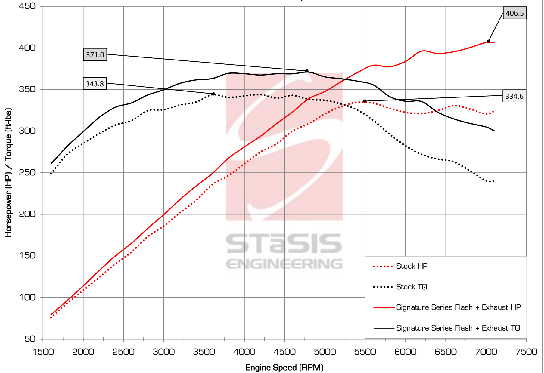
S5 Cabriolet ECU Flash Comparison - Crankshaft Power
