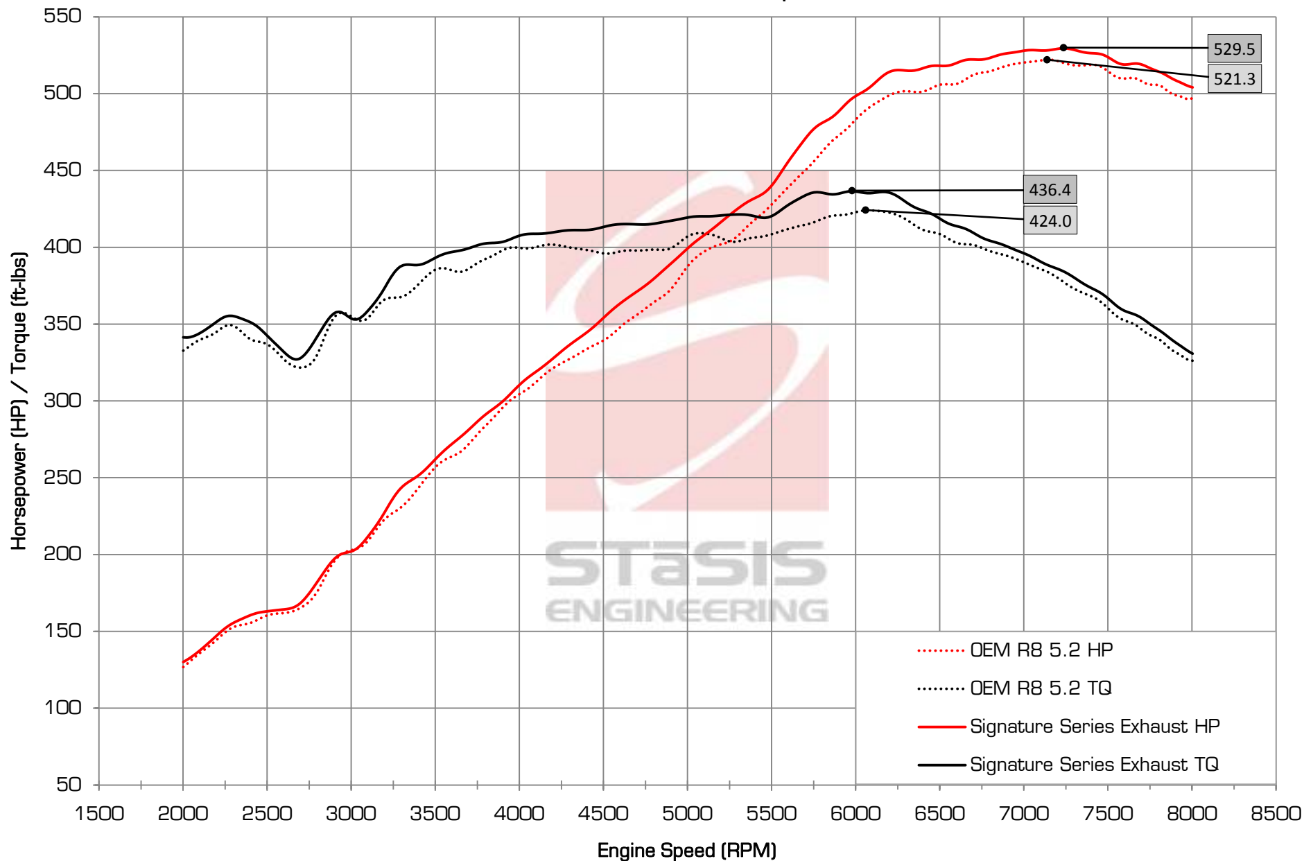
R8 5.2 STaSIS Exhaust Comparison
